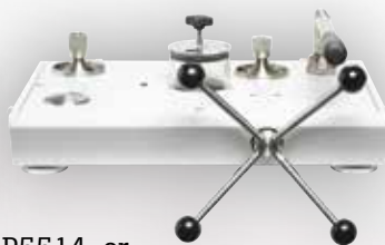
P5514, or P5515 Hydraulic Pressure Comparator
